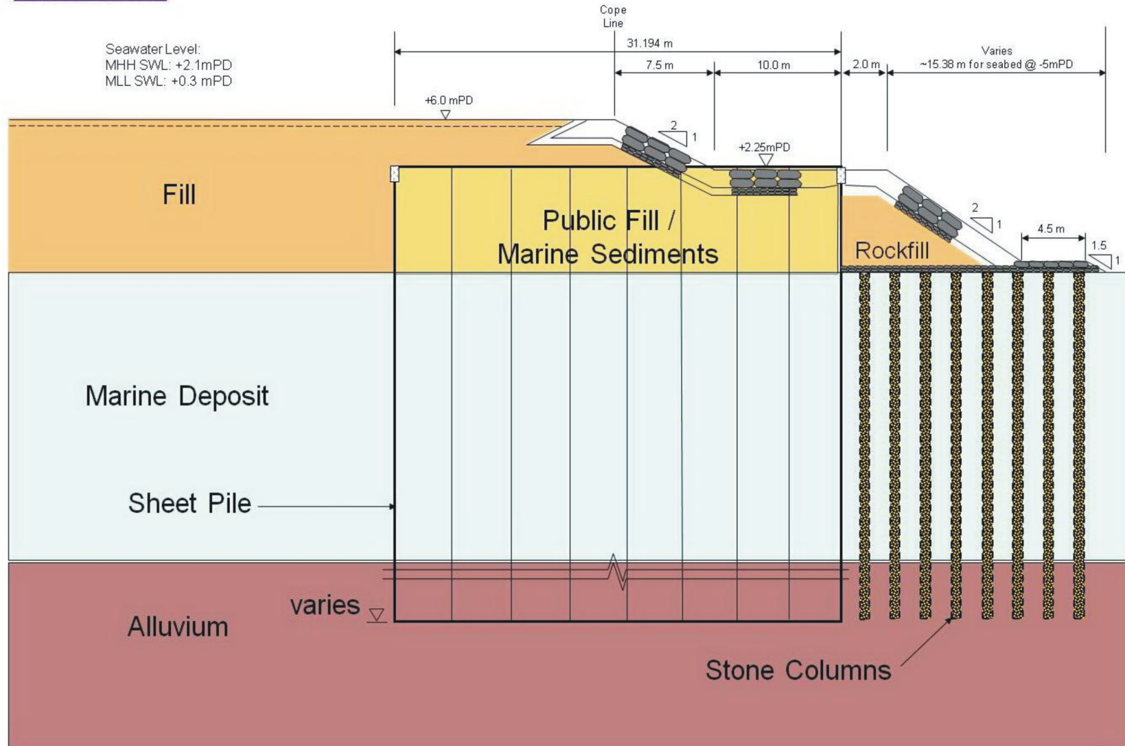
Figure 27 - Schematic Diagram for Seawall Cross-section
